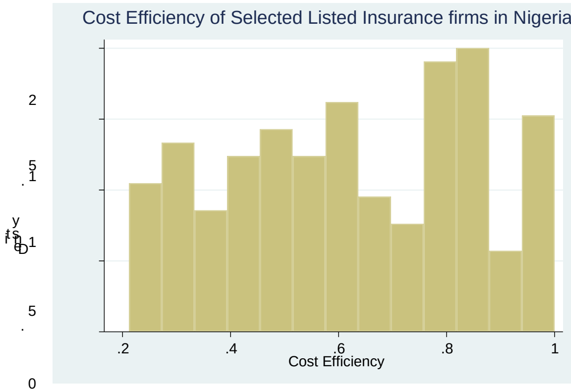
Figure 4.1: Cost Efficiency
